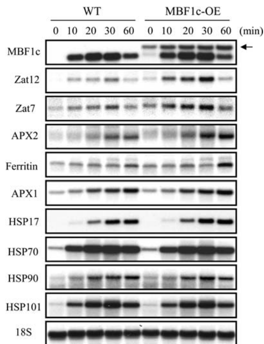
Figure 4. Augmented response of MBF1c-expressing plants (MBF1c-OE) to heat stress. A time-course RNA gel-blot analysis of 2-week-old wild-type and MBF1c-expressing plants subjected to heat stress (38°C, 10, 20, 30, and 60 min), showing the augmented accumulation of transcripts encoding Zat12, Zat7, APX2, and ferritin in transgenic plants. Time-course experiments were repeated three times with similar results. Representative RNA blots are shown. RNA blots and stress assays were performed as described in "Materials and Methods." Plants were grown at 21°C, 14-h light cycle, 100 \mu\text{mol m}^{-2} \text{s}^{-1} , and a relative humidity of 70% and subjected to heat stress as described above. Arrow on right side of top section indicates the transgenic transcript of MBF1c. **, Student's t test significant at P < 0.01 .
