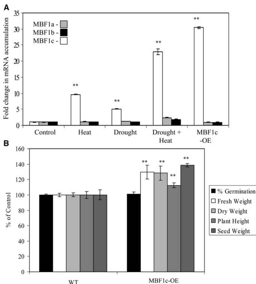
Figure 1. Characterization of transgenic plants expressing MBF1c (MBF1c-OE). A, Relative expression of MBF1 transcripts (MBF1a, At2g42680; MBF1b, At3g58680; MBF1c, At3g24500) in transgenic plants expressing MBF1c (MBF1c-OE) or wild-type plants subjected to heat stress, drought, or a combination of heat stress and drought (after Rizhsky et al. [2004b]). B, Growth and productivity of wild-type and MBF1c-expressing (MBF1c-OE) transgenic plants. Plants were grown at 21°C, 14-h light cycle, 100 \mu\text{mol m}^{-2} \text{s}^{-1} , and a relative humidity of 70%. Production of transgenic plants and RNA blots were performed as described in "Materials and Methods." **, Student's t test significant at P < 0.01 .
