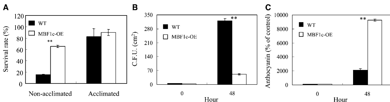
Figure 2. Enhanced tolerance of transgenic plants expressing MBF1c (MBF1c-OE) to heat stress and bacterial growth. A, Survival rates of wild-type and transgenic seedlings in response to heat stress (45°C for 2 h), showing enhanced basal thermotolerance of MBF1c-expressing plants. B, In planta bacterial population measurements showing enhanced resistance of MBF1c-expressing plants to Pseudomonas syringae inoculation. Bacteria (50 cfu \text{cm}^{-2} prepared in water) was infiltrated into leaves with a syringe. Forty-eight hours after inoculation, bacteria was extracted from leaves, plated on agar plates, and scored for cfu \text{cm}^{-2} . C, Augmented accumulation of anthocyanins in MBF1c-expressing plants in response to light stress (1,000 \mu\text{mol m}^{-2} \text{s}^{-1} for 48 h). Stress assays and pathogen infection were performed as described in "Materials and Methods." **, Student's t test significant at P < 0.01 .
