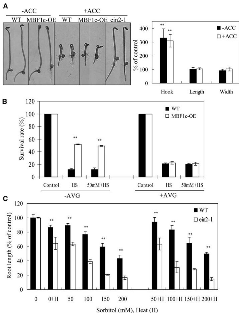
Figure 5. Enhanced tolerance to abiotic stress in MBF1c-expressing plants is mediated by ethylene signaling. A, Triple-response phenotype of etiolated MBF1c-expressing seedlings in the presence or absence of ACC compared to wild type. B, Survival rate measurements showing suppression of MBF1c-induced tolerance to abiotic stress by the ethylene-signaling inhibitor AVG. C, Root growth measurements of ein2 seedlings, impaired in ethylene sensing, showing enhanced sensitivity to osmotic and heat stress compared to wild type. Stress assays, application of AVG, and ein2 analysis were performed as described in "Materials and Methods." **, Student's t test significant at P < 0.01 .
