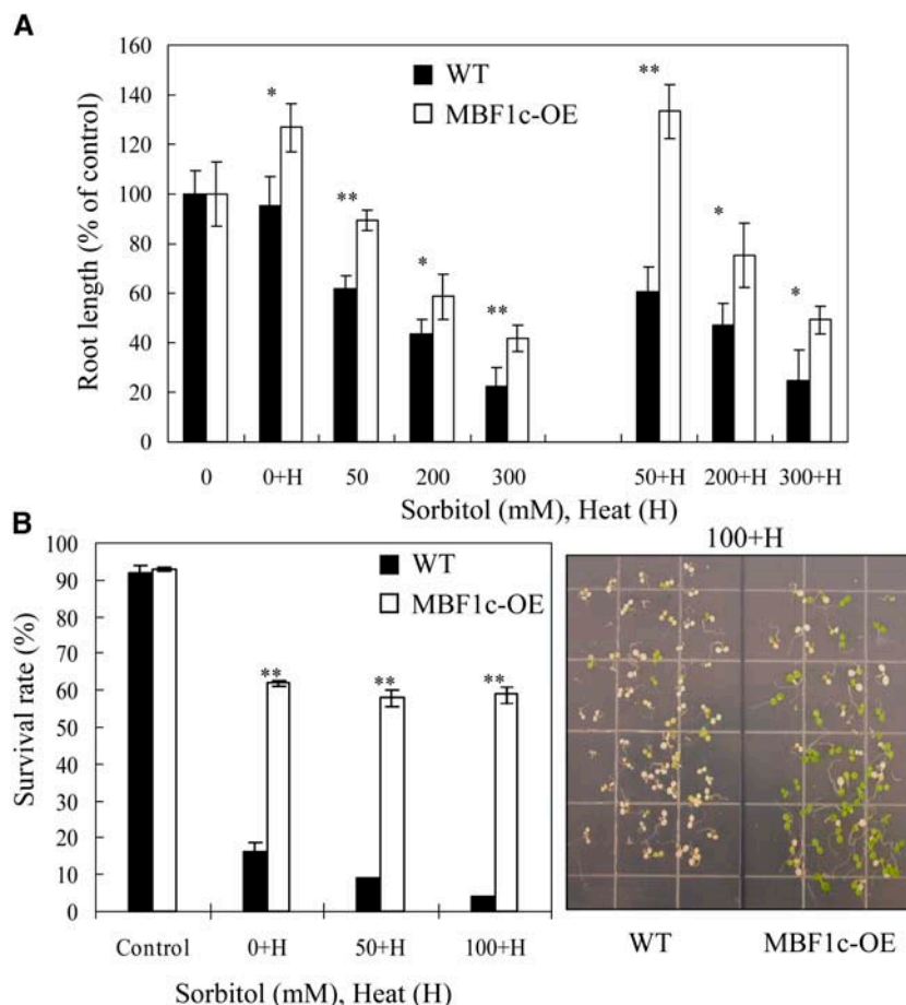
Figure 3. Enhanced tolerance of transgenic seedlings expressing MBF1c (MBF1c-OE) to heat stress, osmotic stress, or a combination of osmotic and heat stress. A, Root growth of wild-type and transgenic seedlings subjected to heat stress (38°C, 48 h), osmotic stress (sorbitol, 50, 200, and 300 mM), or their combination. B, Survival rate measurements of MBF1c-expressing seedlings subjected to heat stress (45°C for 2 h) or heat stress combined with osmotic stress (sorbitol, 50, 100 mM). C, A photograph of wild-type and transgenic seedlings subjected to heat stress (45°C for 2 h) combined with osmotic stress (sorbitol, 100 mM). Stress assays were performed as described in "Materials and Methods." **, Student's t test significant at P < 0.01 ; *, Student's t test significant at P < 0.05 .
